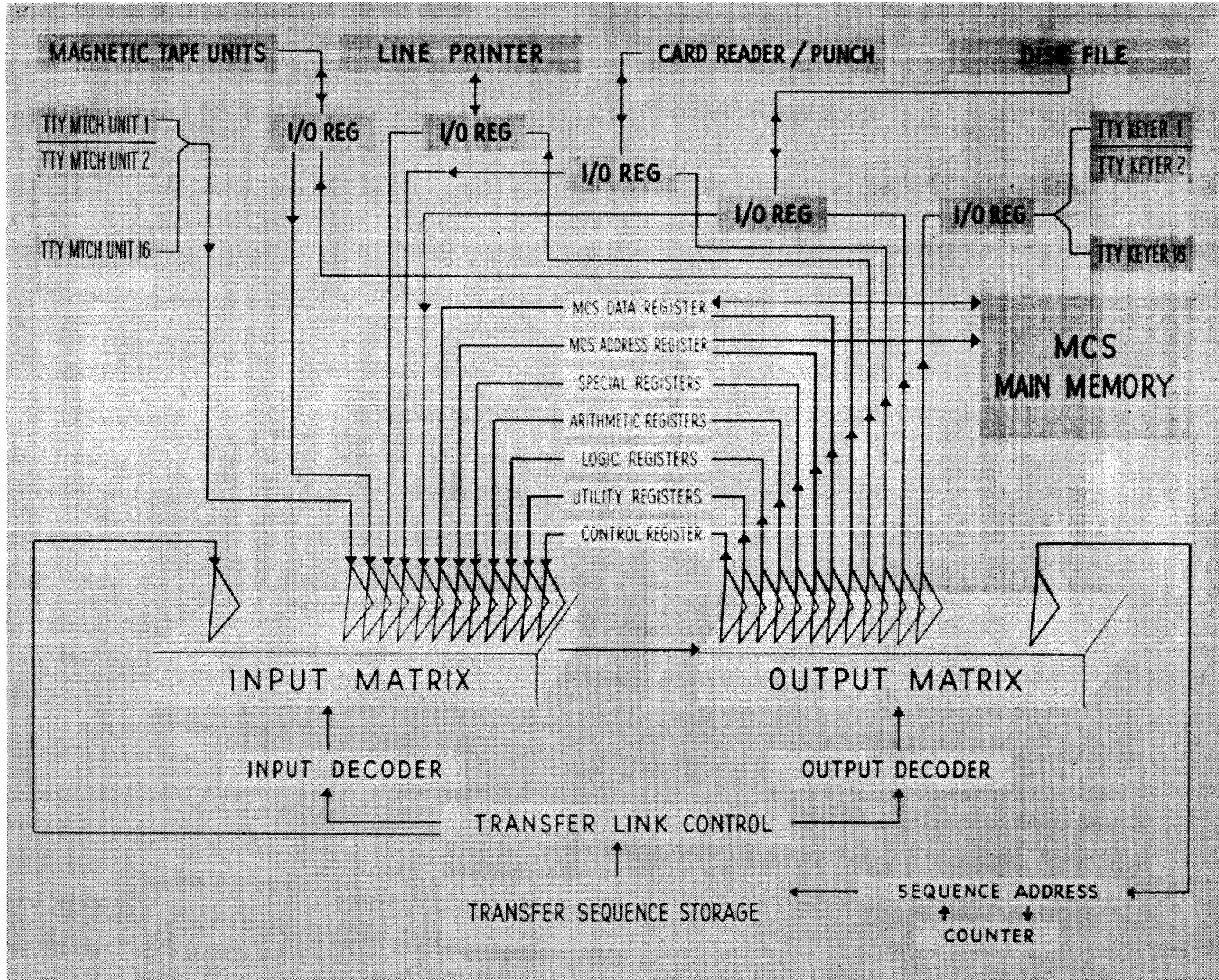
Figure 2. COLLINS C-8401 PROCESSOR ORGANIZATION
