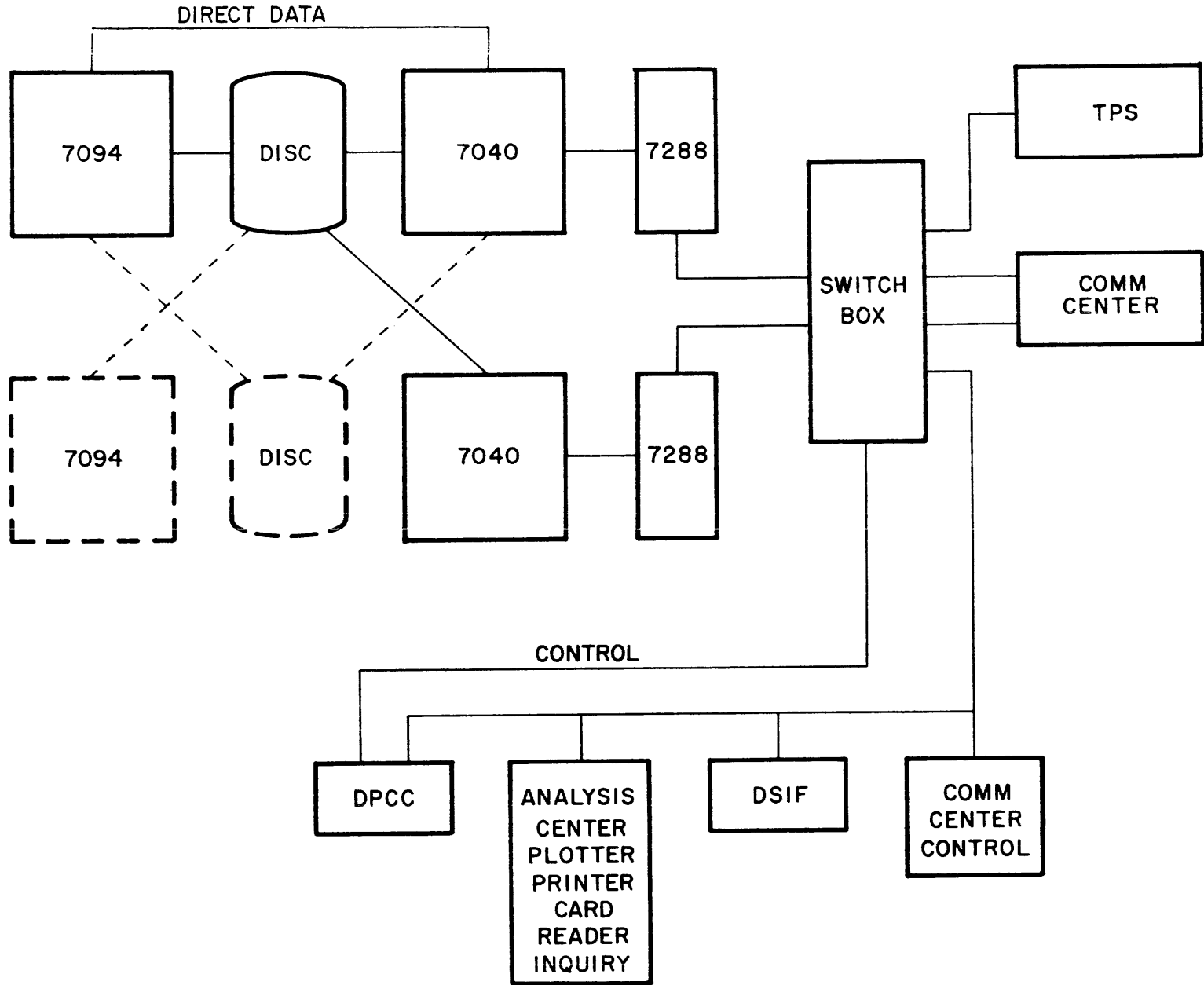
Figure 2. HARDWARE SYSTEM
