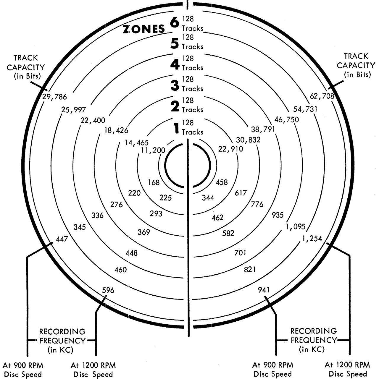
Figure 5. MAXIMUM CAPACITIES OBTAINED WITH SIX-ZONE DISC FORMAT
