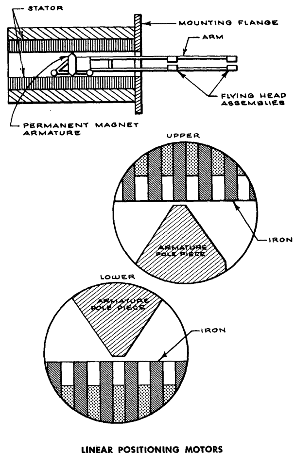
LINEAR POSITIONING MOTORS
