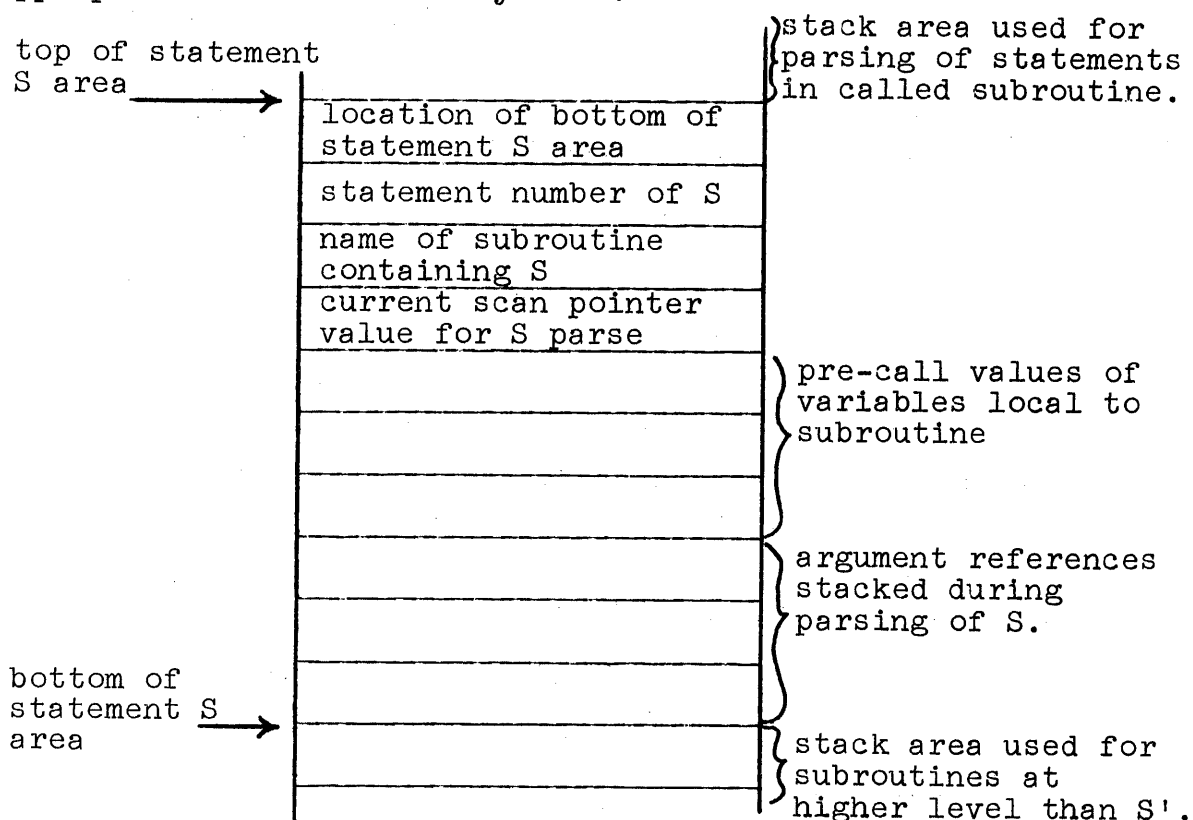
Figure 7. Layout of argument-stack information during a call from a statement to a subroutine.
