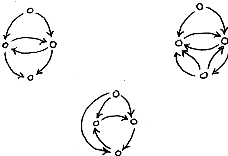
Figure Various irreducible program graphs.
