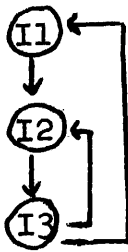
Figure 3. Derived graph of the graph of Figure 2.
