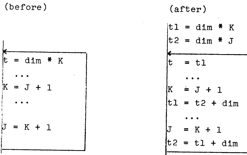
Figure 26. A more elaborate case of reduction in strength.
