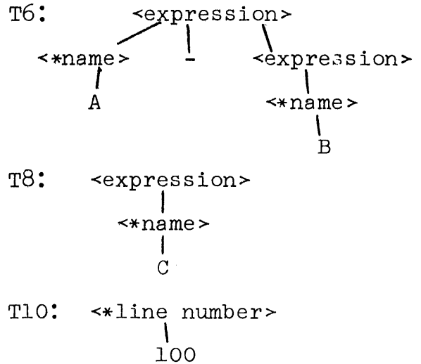
Figure 10. if a - b > c then 100
