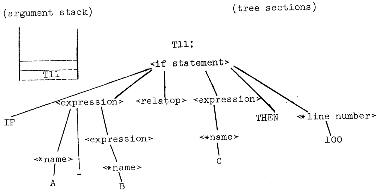
Figure 11. if a - b > c then 100
