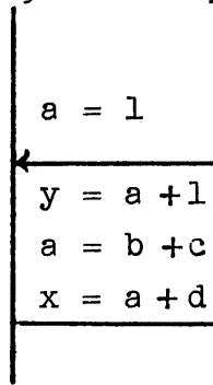
Figure 9A. Expression renaming during motion of code out of a loop.
