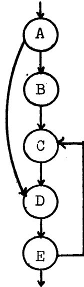
Figure 7. Loop entered by a forward branch.
