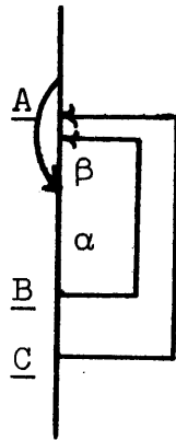
Figure 8A. Code motion out of loops entered by forward branches.
