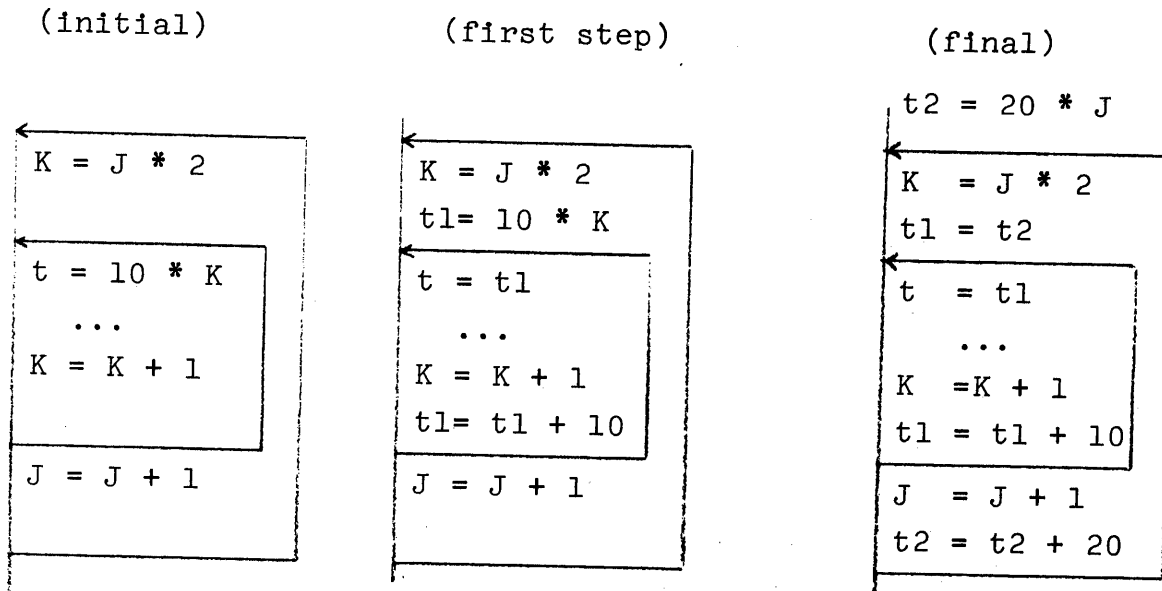
Figure 29. Iterated strength reduction in a nest of loops.
